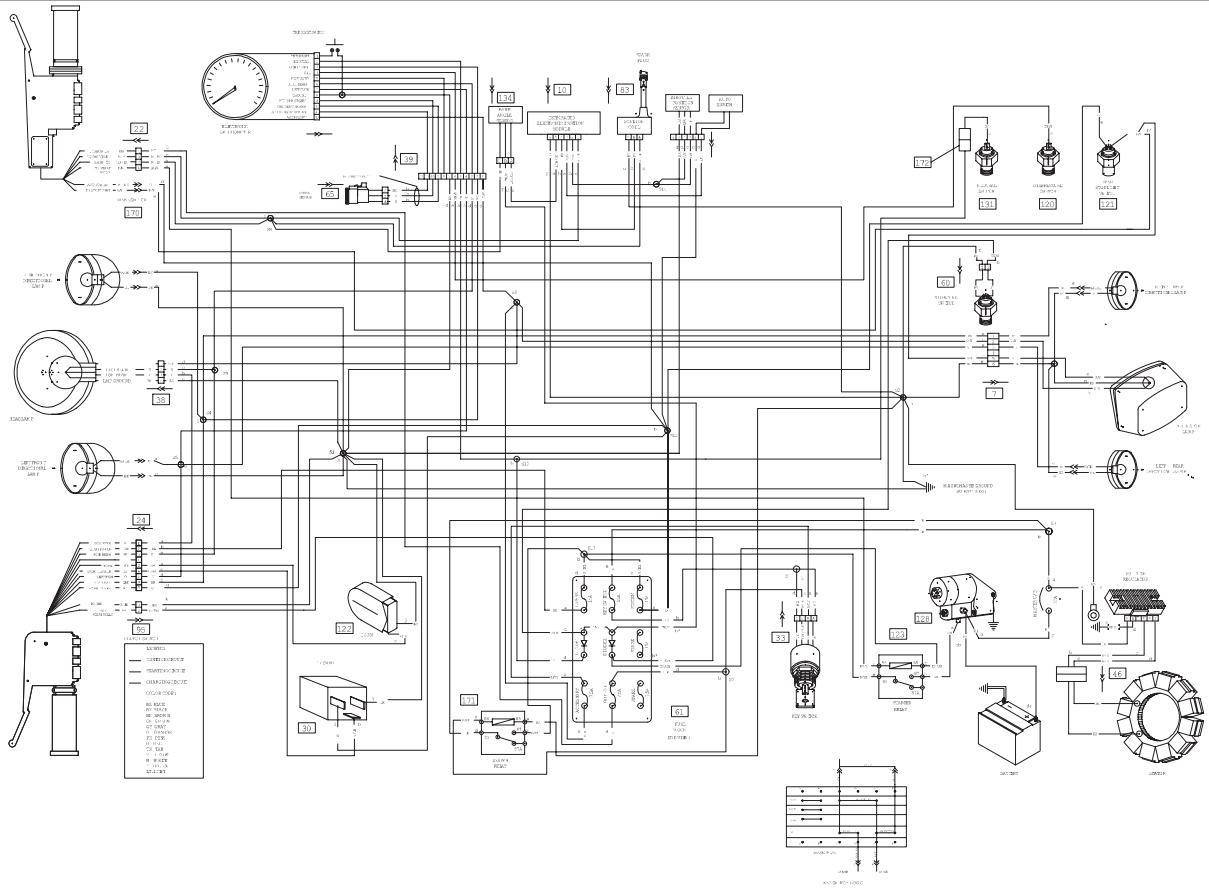
Figure B-10. 2005 Buell Blast P3 Model - Main Harness
